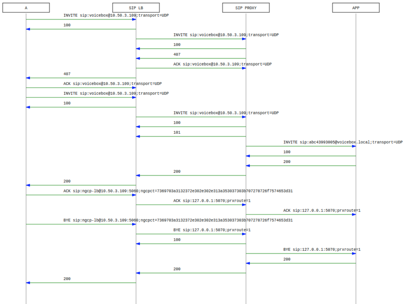
Figure 229. Voicebox Call-Flow
