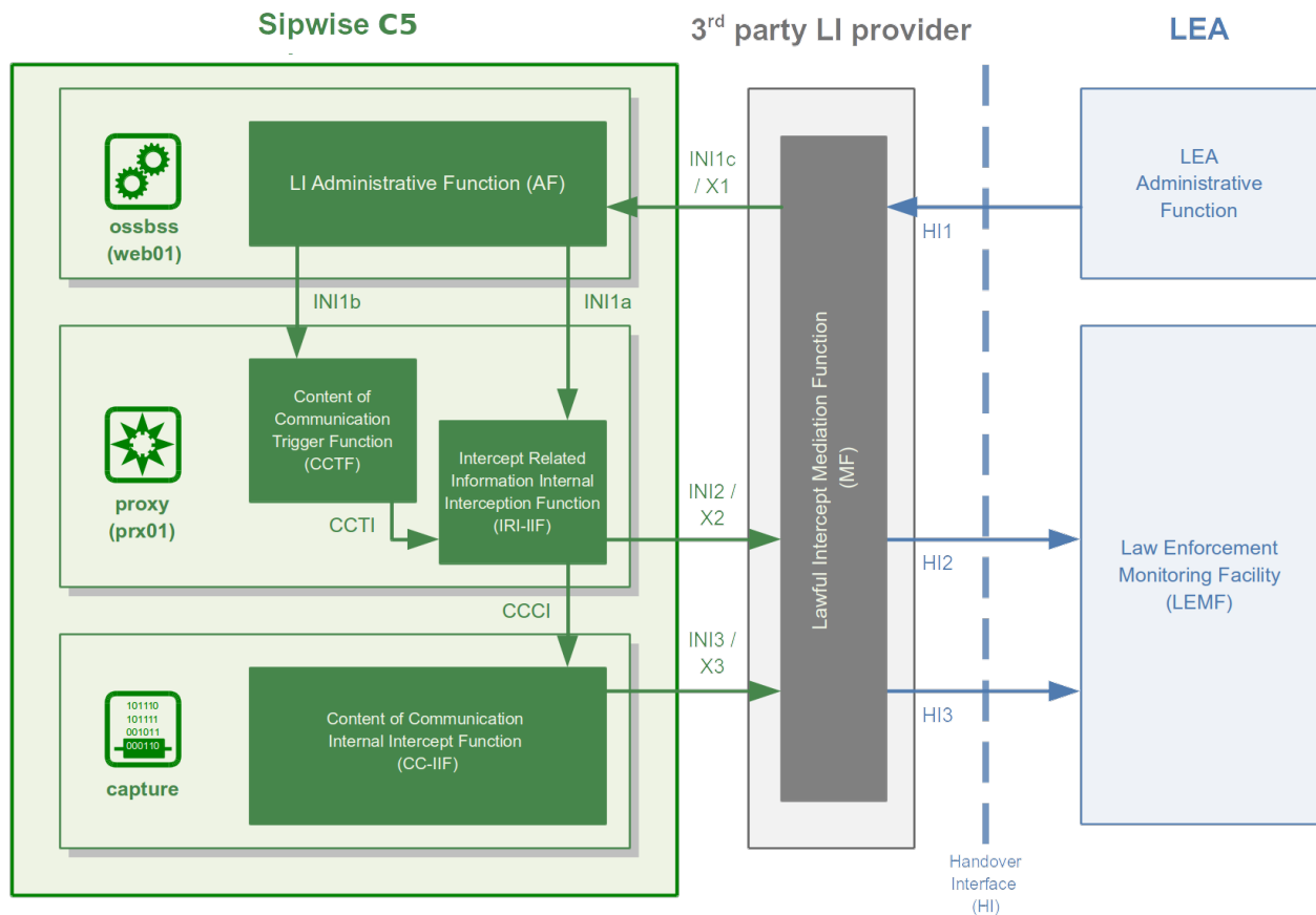
Figure 167. LI with 3rd Party Provider
