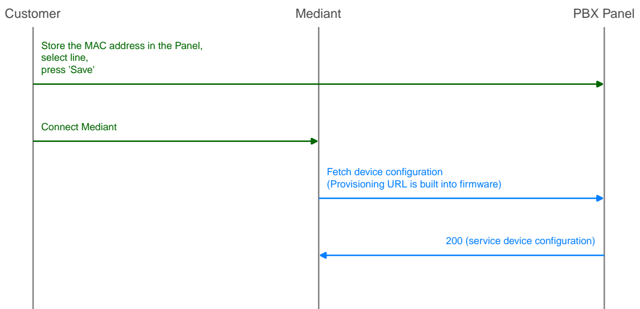
Figure 154. Initially bootstrap a Mediant gateway
