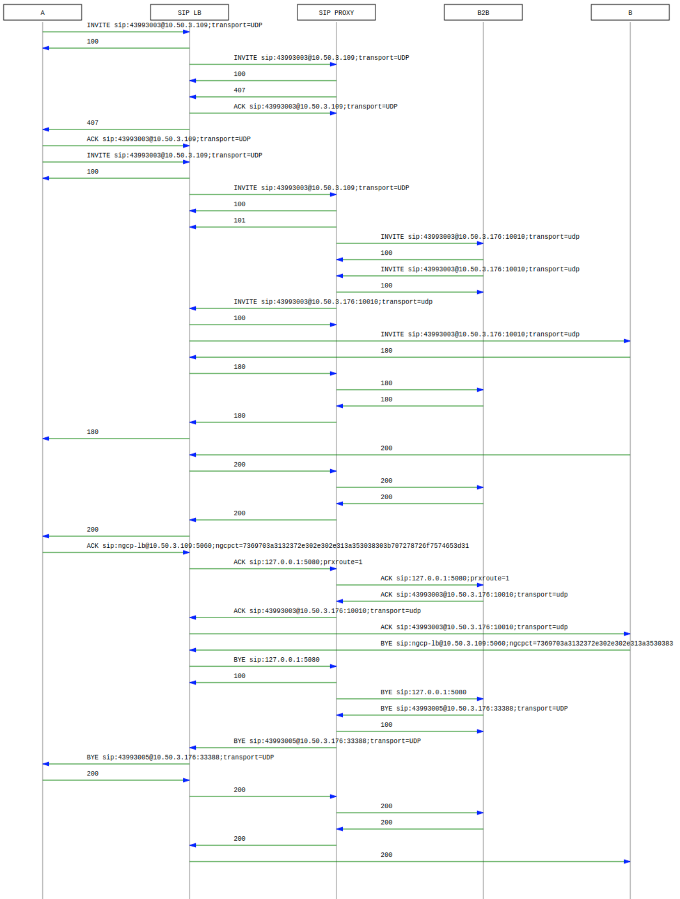
Figure 191. Basic Call Call-Flow
