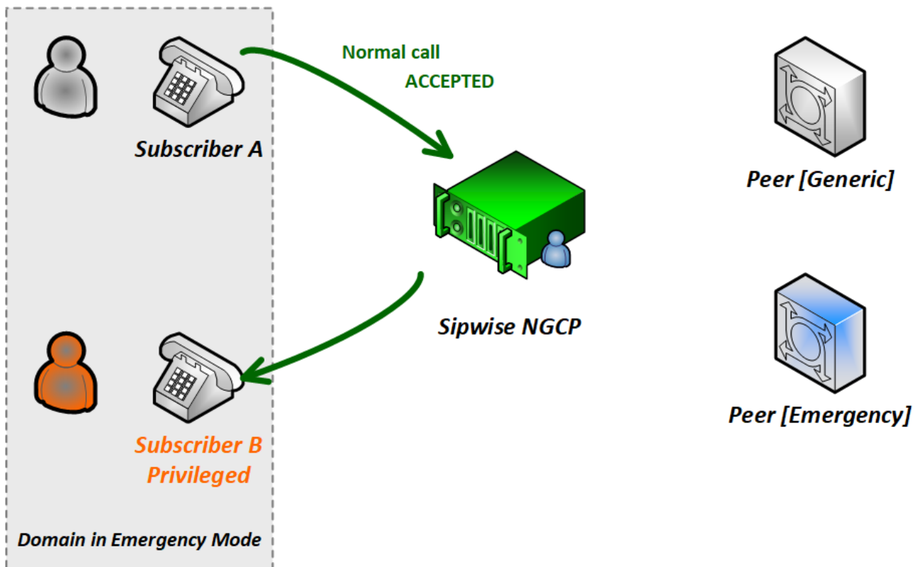
Figure 86. Call-flow in Emergency Mode 3. (Std to Priv)
