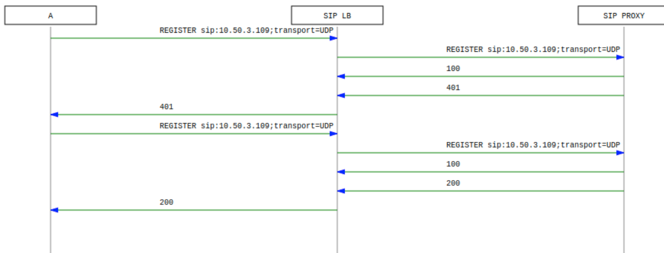
Figure 190. Registration Call-Flow
