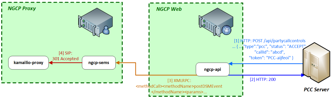
Figure 172. Call Accepted by PCC
