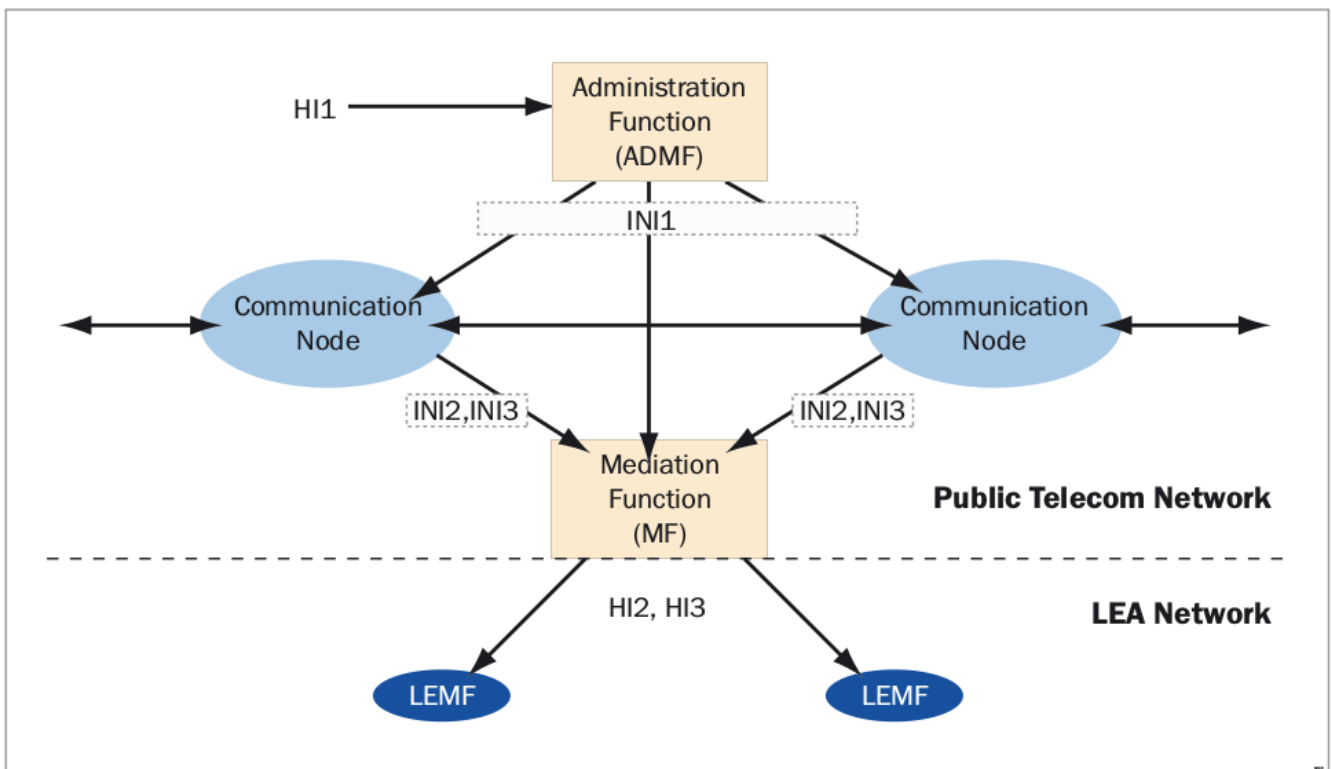
Figure 166. LI: ETSI Interfaces
