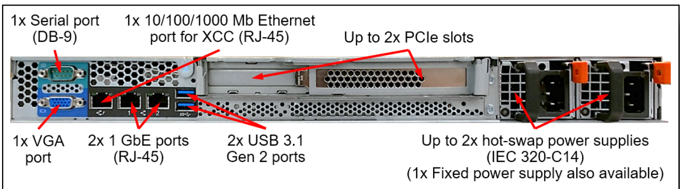
Figure 16. Lenovo SR250 Rear View
