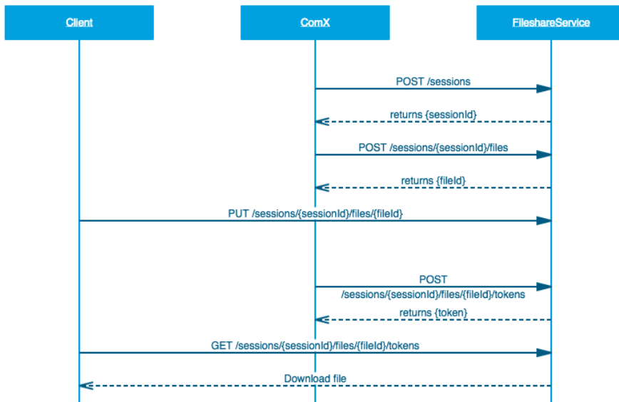
Figure 180. Sequence Simple
