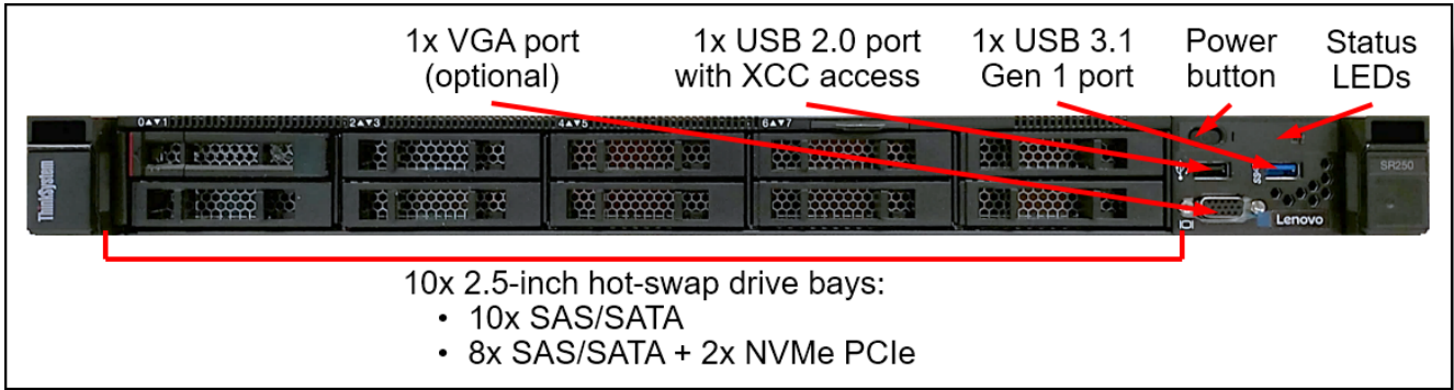
Figure 14. Lenovo SR250 Front View
