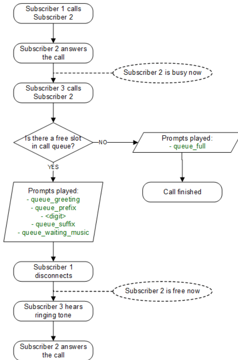
Figure 148. Flowchart of Call Queue
